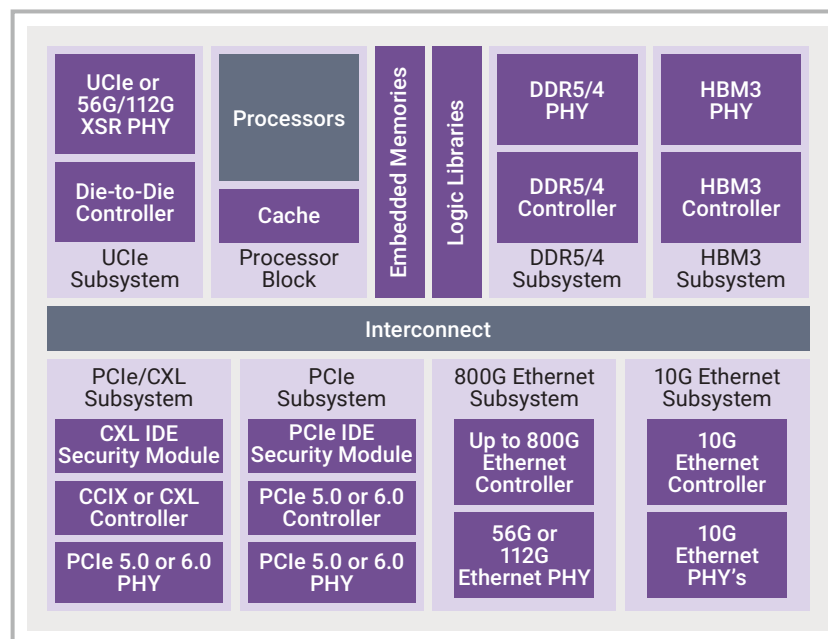
Figure 1: IP Accelerated SoC Subsystem Solutions
